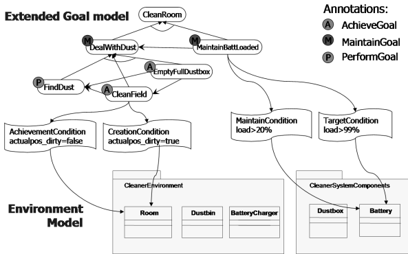
Figure 1. Goal model and Environmental model, with the correlations between them.
